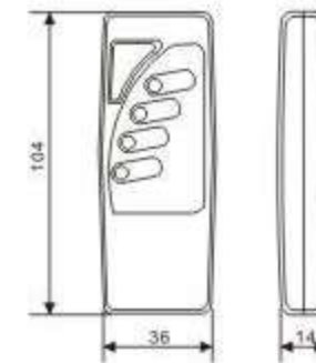
Dimensioned Drawing for Remote Control
